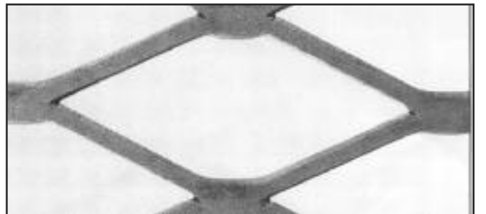
1-1/2" #9 FLATTENED
